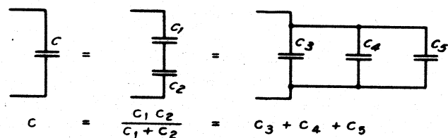
Fig. 14. Combinations of capacitors which give resultant capacitances equal to that of a single capacitor are shown here with the resultant capacitance of each combination listed below it.
