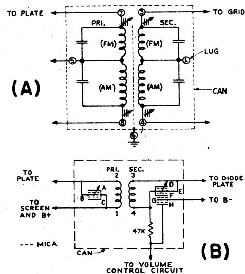
Fig. 1-15. (A) An i-f transformer of the dual-frequency variety found in a-m—f-m receivers. The a-m and f-m windings of the i-f transformer are in series and are contained in the same can; in (B) is shown a unit which contains, besides the i-f transformer, the filter capacitors and trimmers used in the associated circuit.
