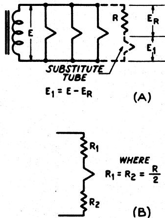
Fig. 1-3. When substituting a tube with lower voltage requirements than the original, a series resistor is added in the branch of the parallel feed in which the tube is placed. The resistor may be a single one as in (A), or two smaller ones as in (B).
