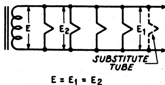
Fig. 1-2. Parallel connection of vacuum-tube heaters. The voltage drops across the heaters so connected are equal to the voltage across the secondary of the power transformer as shown.
