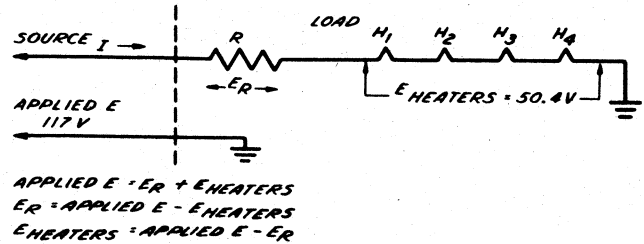
Fig. 1-6. A series chain of four filaments or heaters with a line voltage-dropping resistor. The voltage drop across the line voltage-dropping resistor makes up for the differences between the line voltage and the voltage required by the four heaters.
