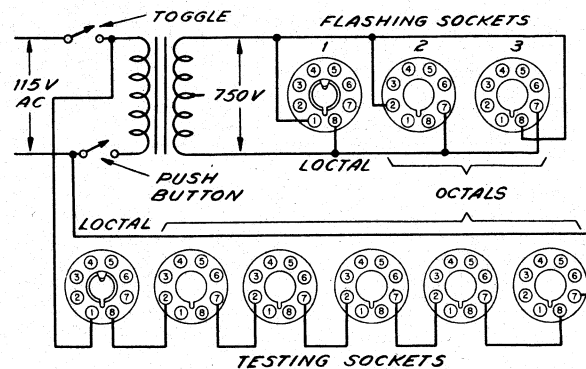
FIG. 4-1. Illustrating the setup for filament repair.
