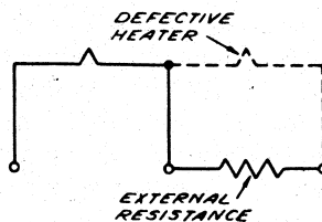
Fig. 1-12. A defective heater in a dual-heater tube may be replaced by an external resistor equal in resistance to the defective element.
