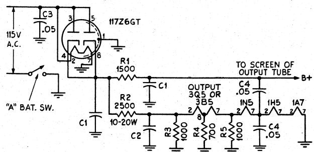
FIG. 4-2. Typical circuit arrangement for changing battery-operated radio to electric operation using a 117Z6GT rectifier tube.
