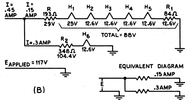
Fig. 1-9(B). H_6 of Fig. 1-9(A) has been replaced by a 12.6-volt, 0.3-ampere one requiring a separate series circuit and an increase in the current drawn from the line source. Now there are two dropping resistors, one in each branch of the circuit.
