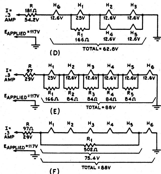
Fig. 1-9(D), (E), and (F). Various methods are shown here for shunting the heaters of the circuit shown in Fig. 1-9(A), after the substitution of a 12.6-volt 0.3-ampere heater for H_6 , so that the voltage and current requirements of each heater are satisfied.
