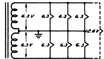
Fig. 1-4. Filament circuit of the type found in many television receivers. The center tap between the two windings is grounded to serve as a return for the filaments in parallel, each of which receives 6.3 volts from its part of the secondary.
